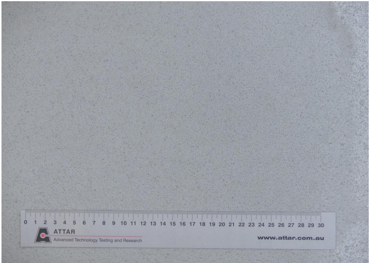
Figure 1: Fosroc Nitoflor PU 200 + Silica Sand (16/30) Broadcast + Fosroc Nitoflor PU 200
